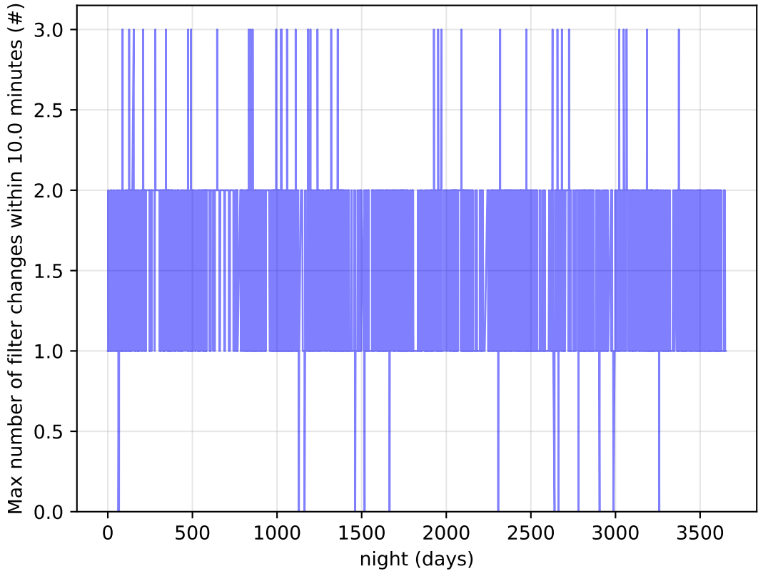
ddf_acor_sf10_Isf20_Isr50_v3.4_10yrs Per Night: Max number of filter changes within 10.0 minutes
