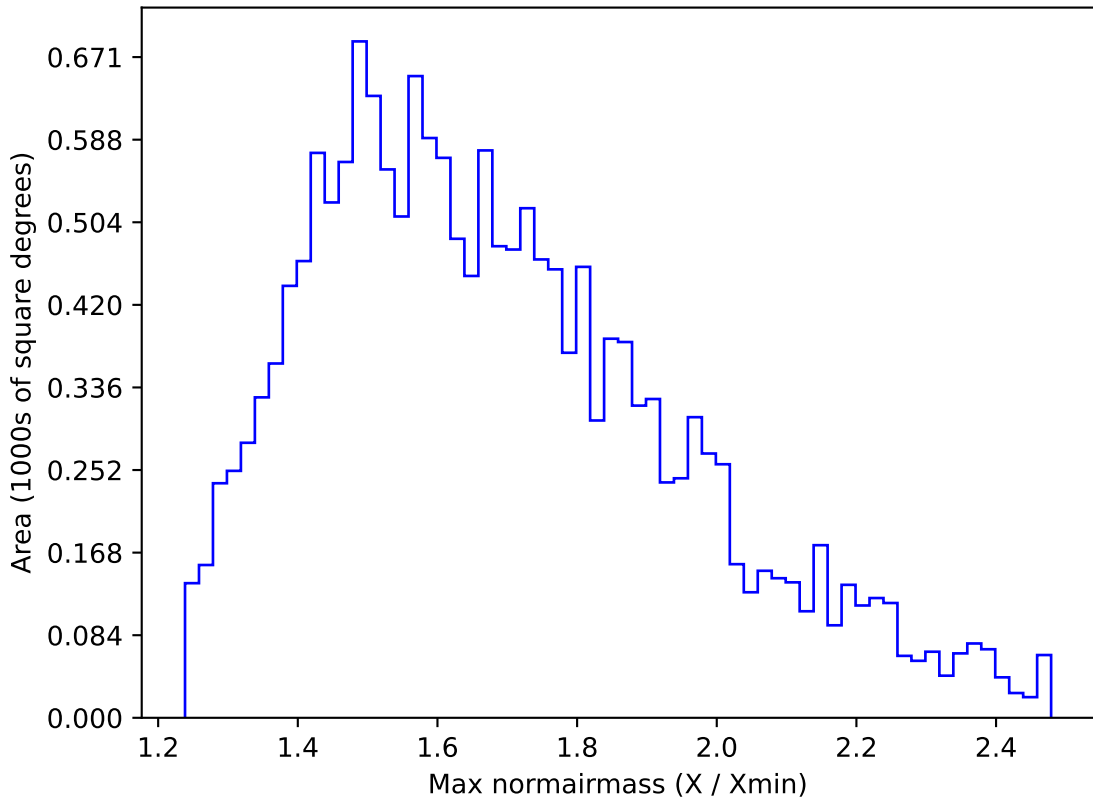
ddf_acor_sf10_lsf20_lsr50_v3.4_10yrs WFD u band: Max normairmass
