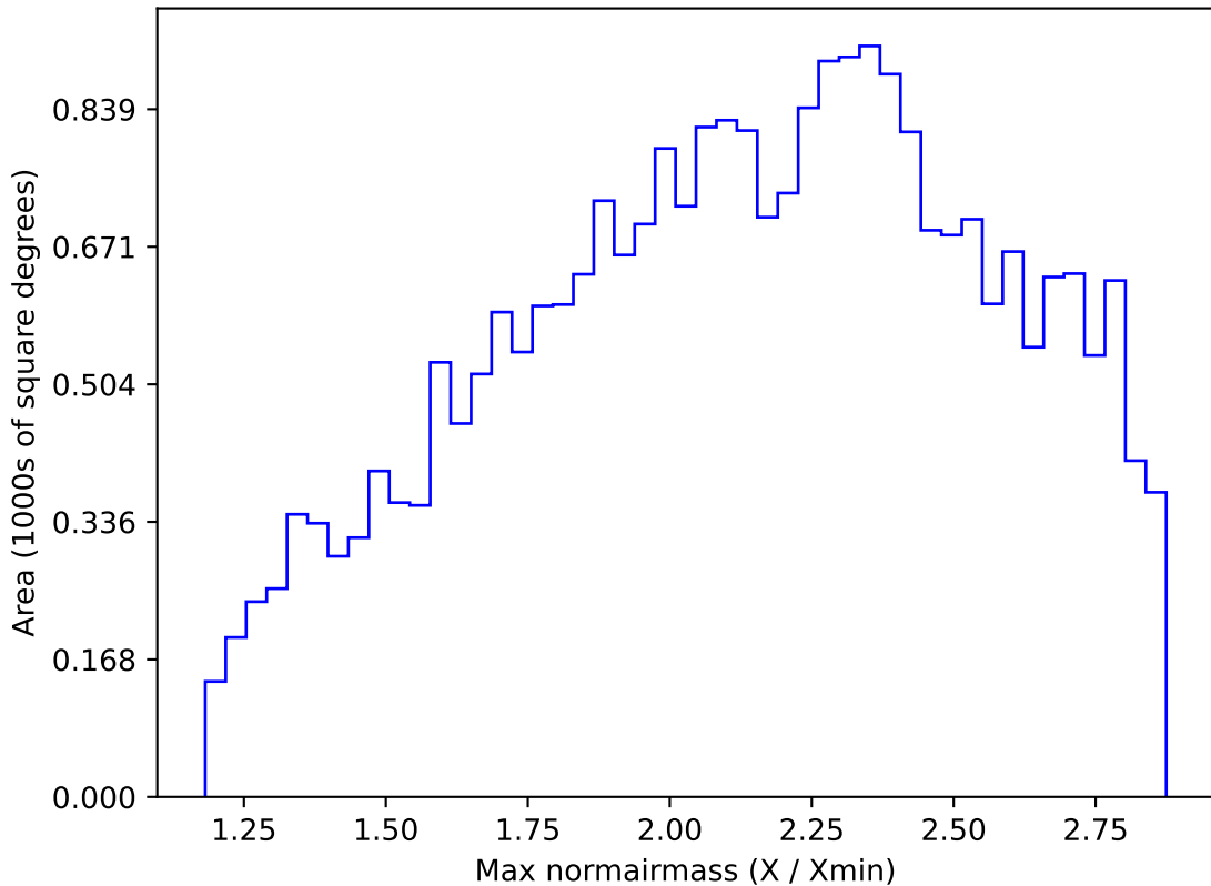
ddf_acor_sf10_lsf20_lsr50_v3.4_10yrs All sky i band: Max normairmass
