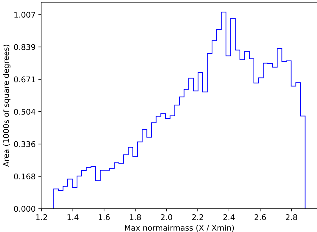
ddf_acor_sf10_lsf20_lsr50_v3.4_10yrs All sky all bands: Max normairmass
