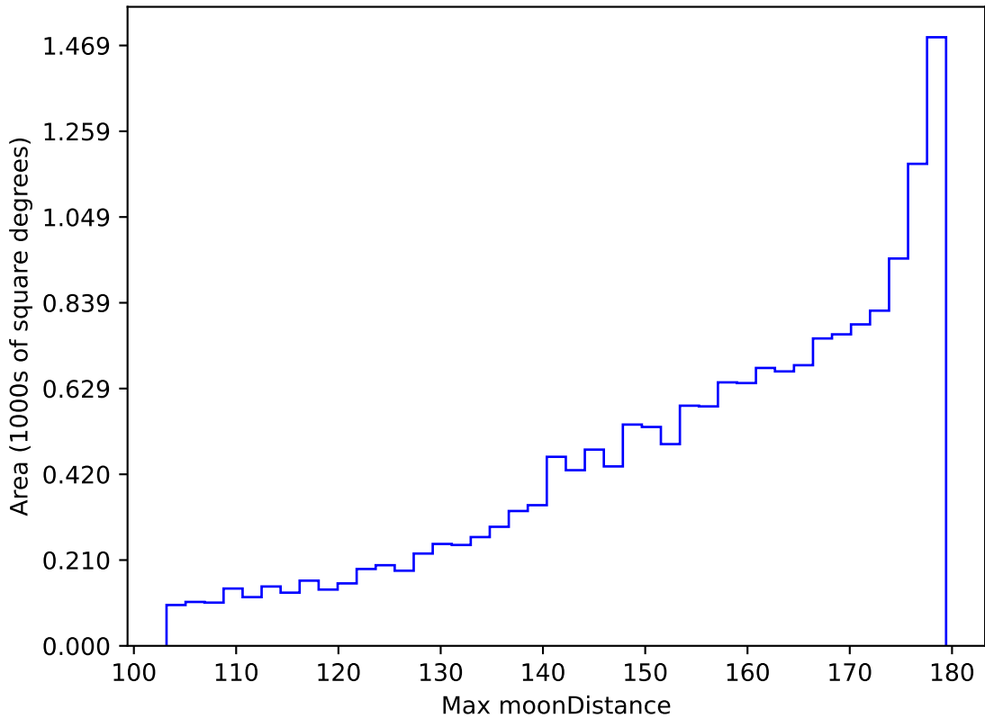
ddf_acor_sf10_lsf20_lsr50_v3.4_10yrs WFD r band: Max moonDistance
