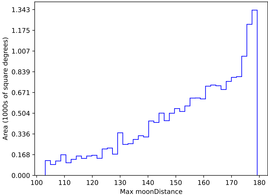
ddf_acor_sf10_lsf20_lsr50_v3.4_10yrs WFD i band: Max moonDistance
