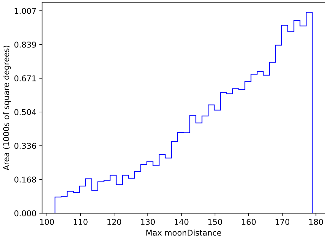
ddf_acor_sf10_lsf20_lsr50_v3.4_10yrs WFD g band: Max moonDistance
