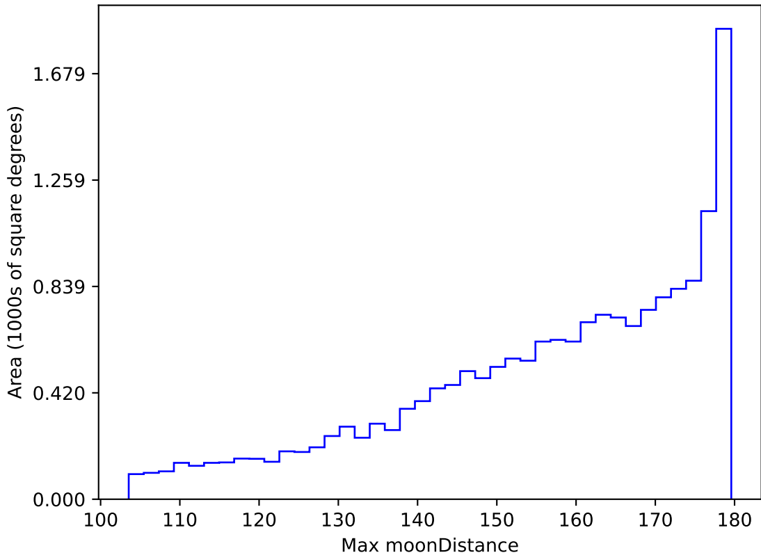
ddf_acor_sf10_lsf20_lsr50_v3.4_10yrs WFD all bands: Max moonDistance
