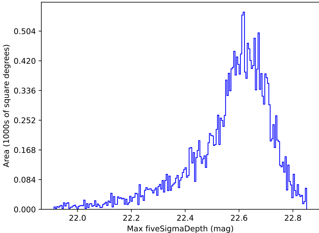
ddf_acor_sf10_ls20_lsr50_v3.4_10yrs All sky y band: Max fiveSigmaDepth
