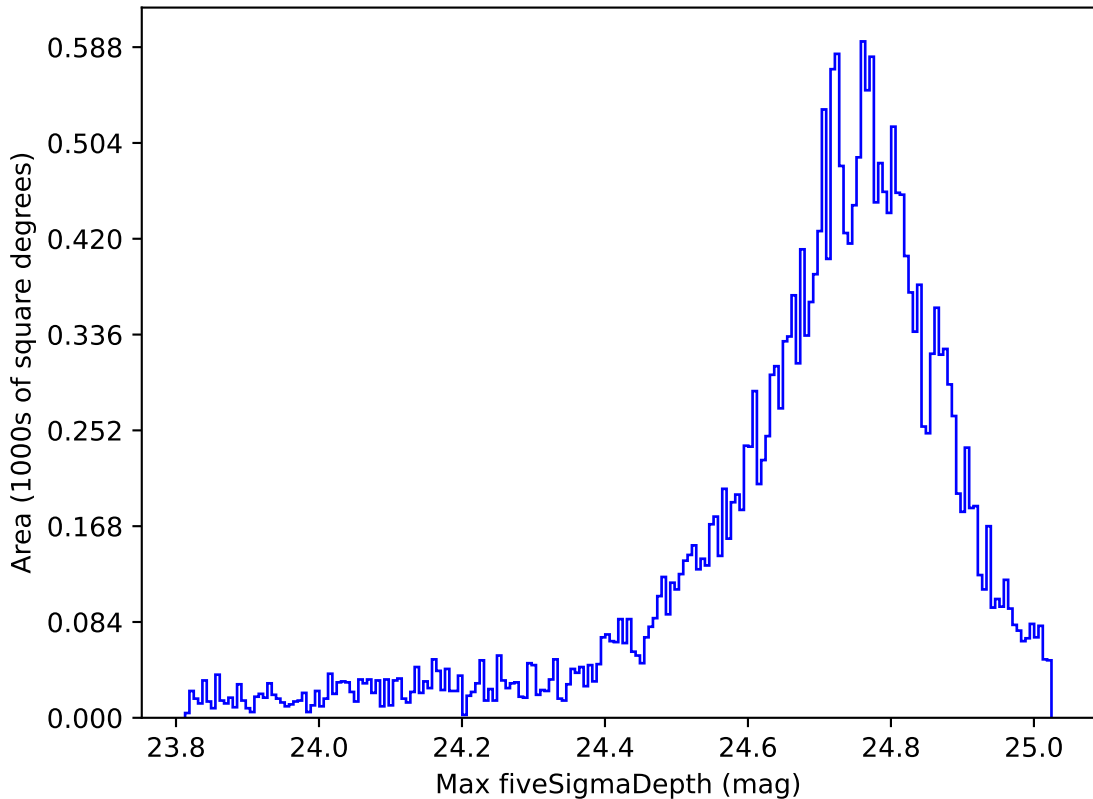
ddf_acor_sf10_lsf20_lsr50_v3.4_10yrs All sky r band: Max fiveSigmaDepth
