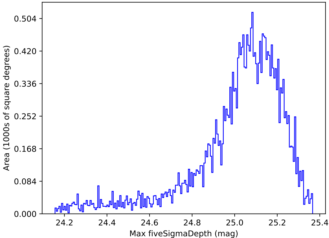
ddf_acor_sf10_ls20_lsr50_v3.4_10yrs All sky g band: Max fiveSigmaDepth
