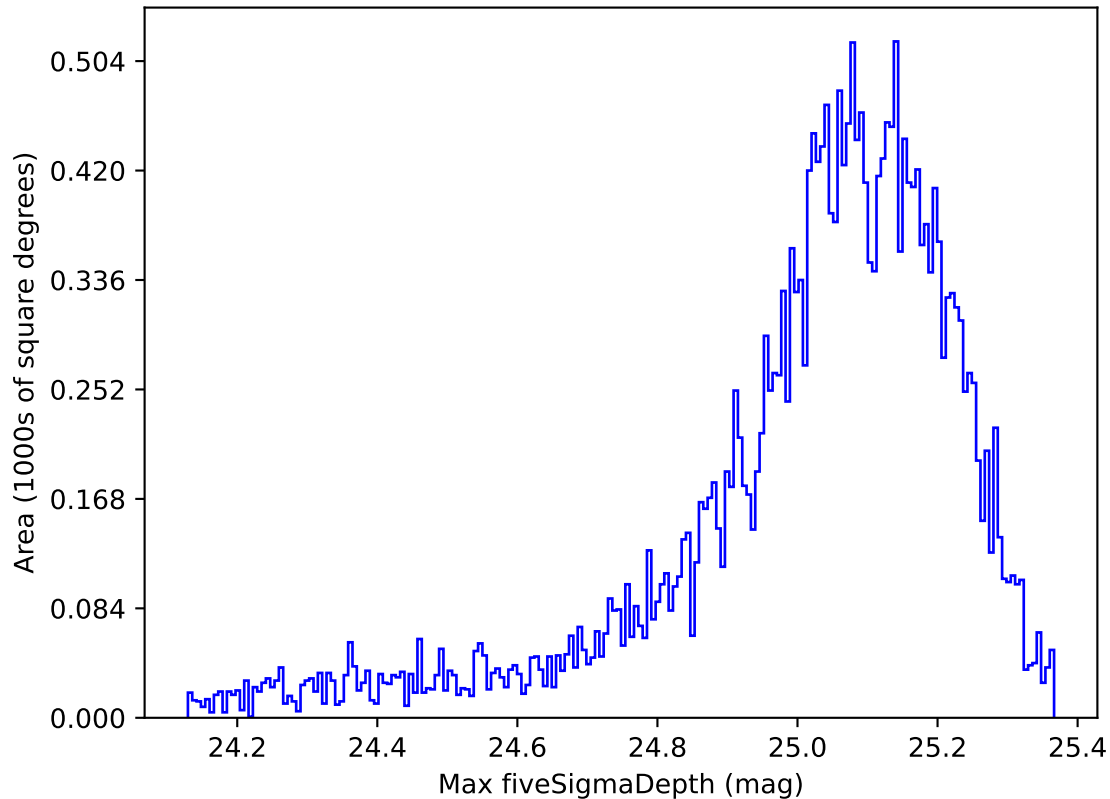
ddf_acor_sf10_lsf20_lsr50_v3.4_10yrs All sky all bands: Max fiveSigmaDepth
