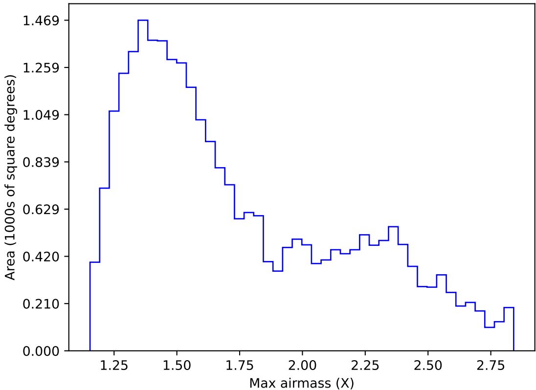
ddf_acor_sf10_lsf20_lsr50_v3.4_10yrs Yr 1 z band: Max airmass
