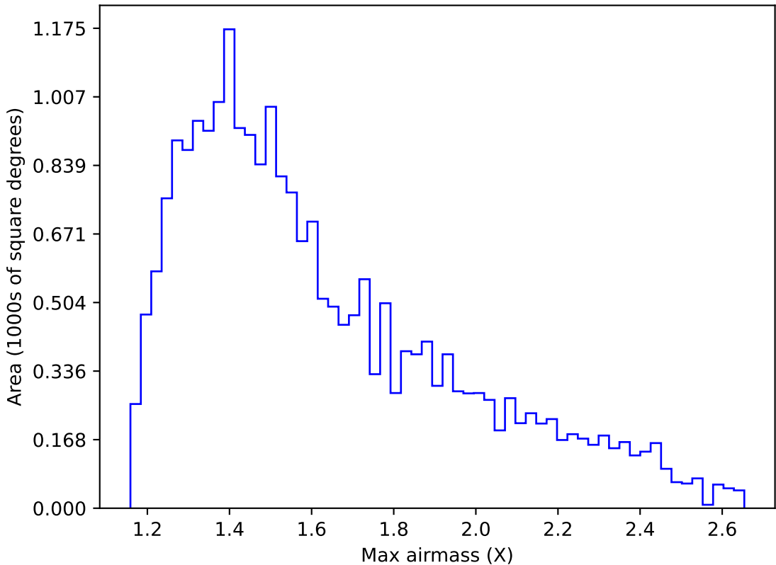
ddf_acor_sf10_lsf20_lsr50_v3.4_10yrs Yr 1 y band: Max airmass
