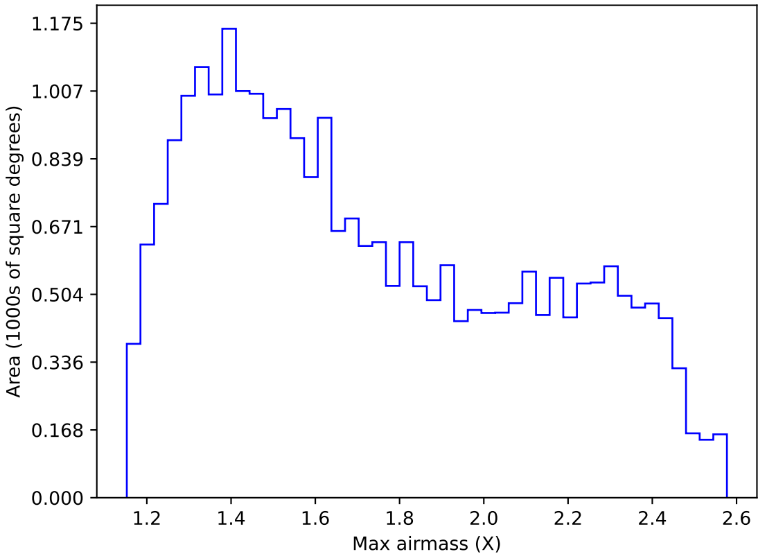
ddf_acor_sf10_lsf20_lsr50_v3.4_10yrs Yr 1 r band: Max airmass
