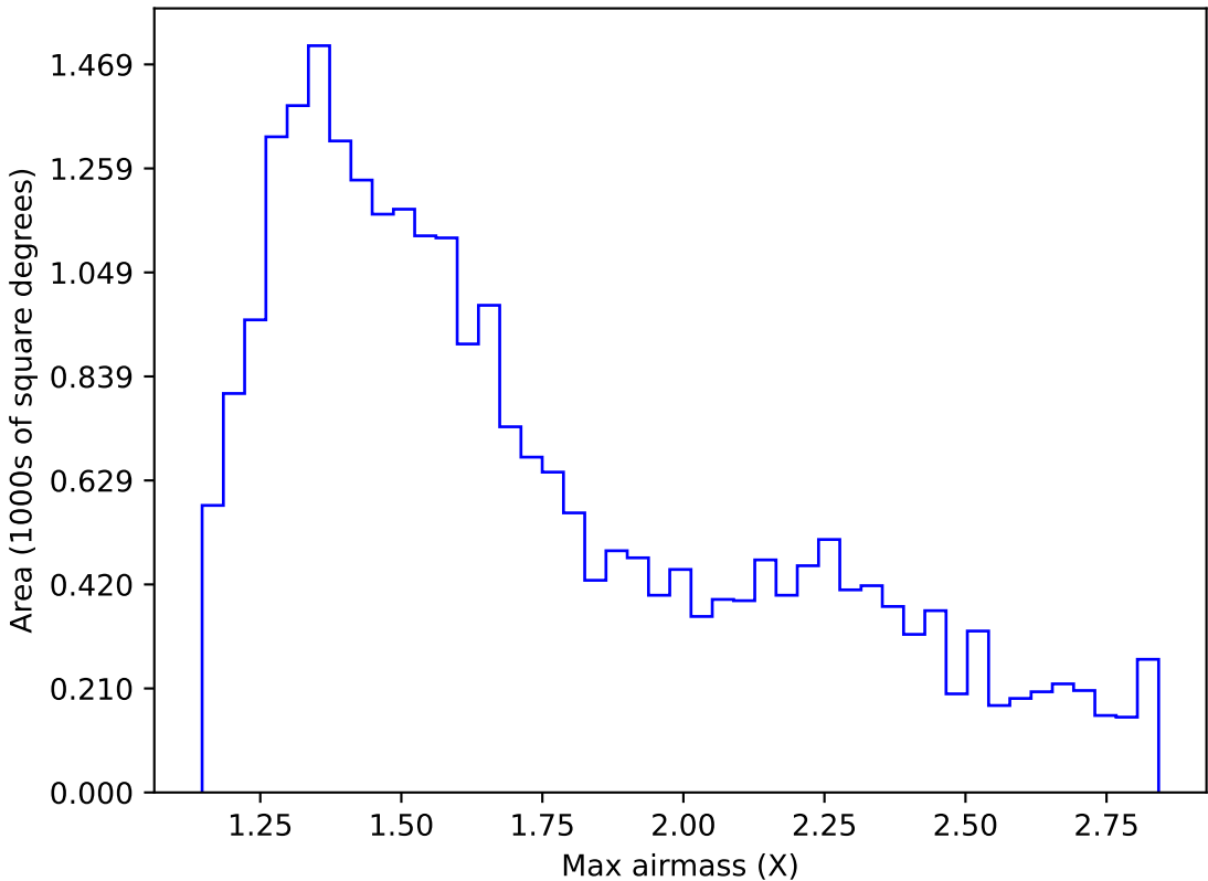
ddf_acor_sf10_lsf20_lsr50_v3.4_10yrs Yr 1 i band: Max airmass
