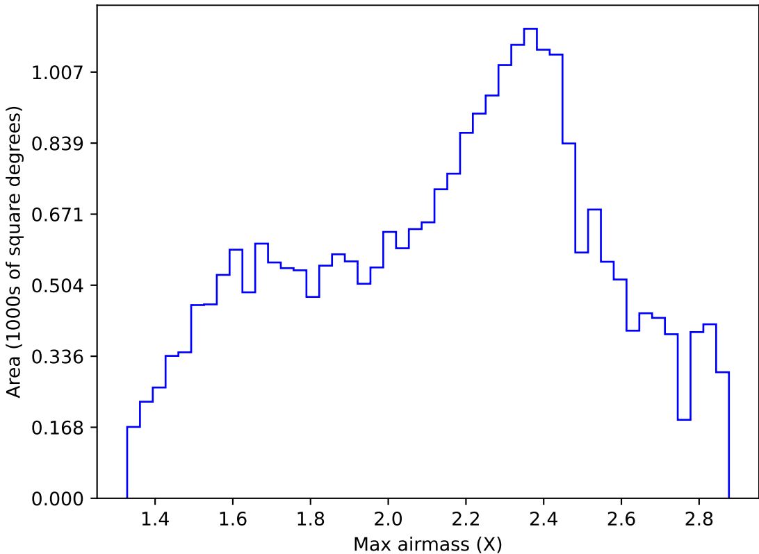
ddf_acor_sf10_lsf20_lsr50_v3.4_10yrs Yr 1 all bands: Max airmass
