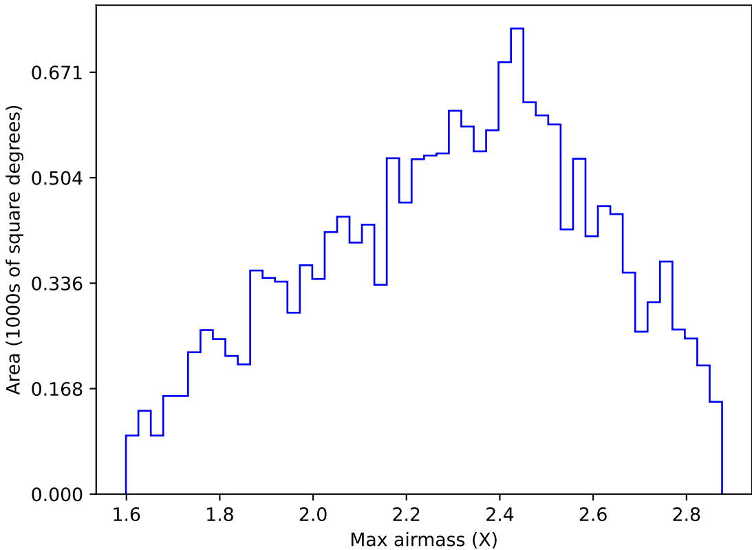
ddf_acor_sf10_lsf20_lsr50_v3.4_10yrs WFD y band: Max airmass
