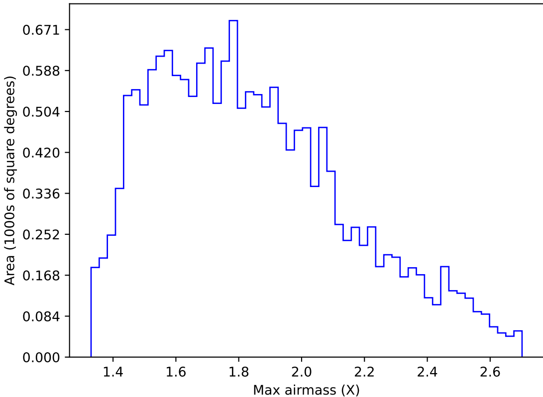
ddf_acor_sf10_lsf20_lsr50_v3.4_10yrs WFD u band: Max airmass
