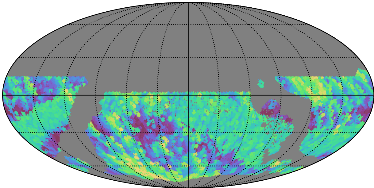
ddf_acor_sf10_lsf20_lsr50_v3.4_10yrs WFD r band: Max airmass
