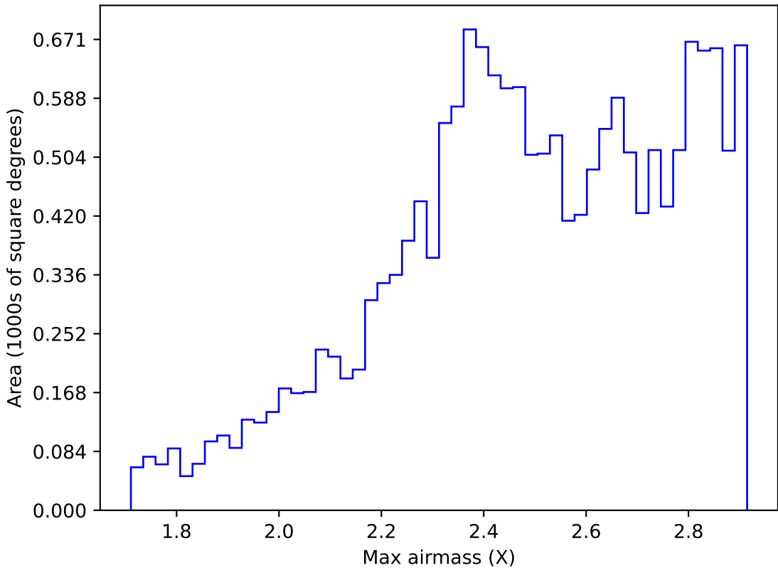
ddf_acor_sf10_lsf20_lsr50_v3.4_10yrs WFD i band: Max airmass
