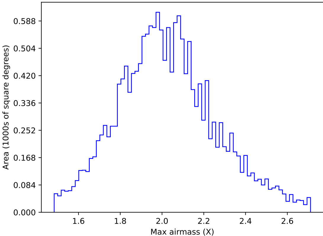
ddf_acor_sf10_lsf20_lsr50_v3.4_10yrs WFD g band: Max airmass
