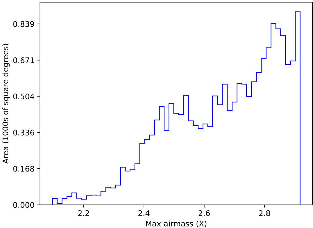
ddf_acor_sf10_lsf20_lsr50_v3.4_10yrs WFD all bands: Max airmass
