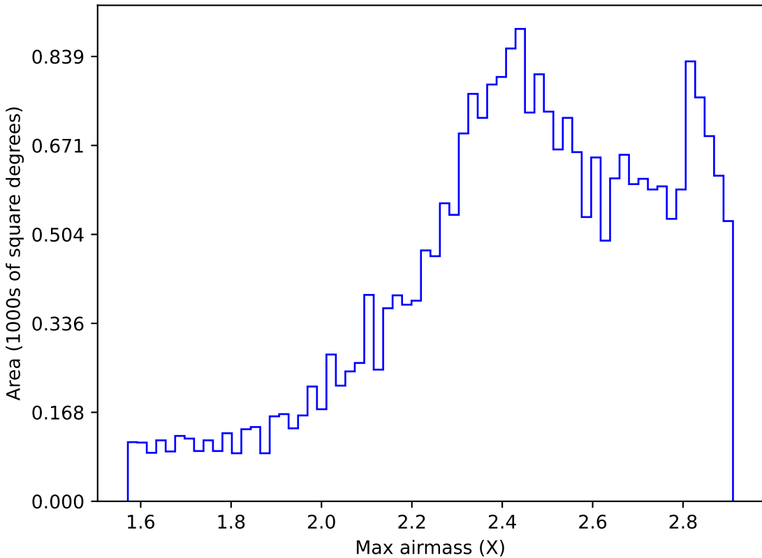
ddf_acor_sf10_lsf20_lsr50_v3.4_10yrs All sky z band: Max airmass
