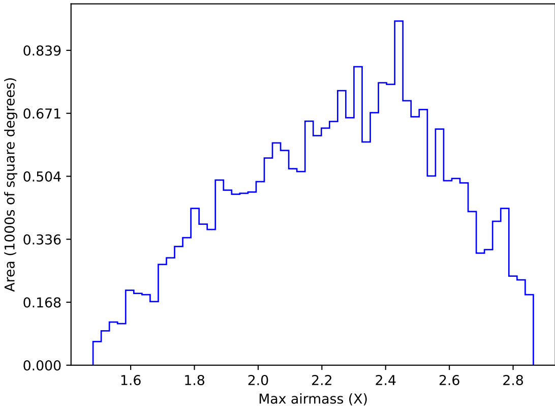
ddf_acor_sf10_lsf20_lsr50_v3.4_10yrs All sky y band: Max airmass
