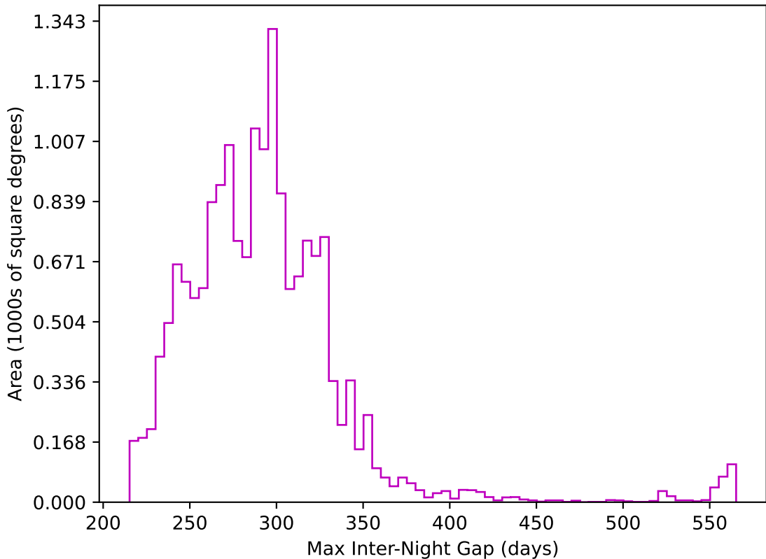
ddf_acor_sf10_lsf20_lsr50_v3.4_10yrs WFD z band: Max Inter-Night Gap
