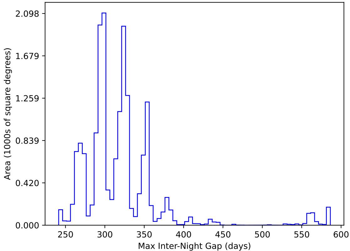
ddf_acor_sf10_lsf20_lsr50_v3.4_10yrs WFD y band: Max Inter-Night Gap
