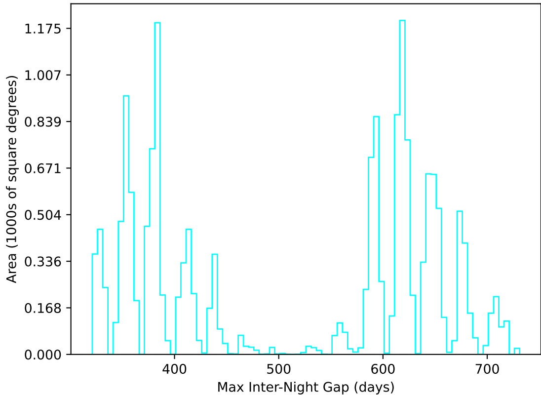
ddf_acor_sf10_lsf20_lsr50_v3.4_10yrs WFD u band: Max Inter-Night Gap
