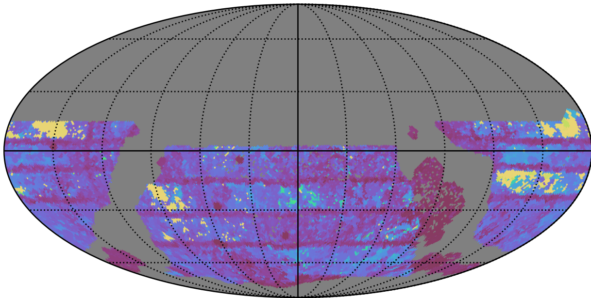
ddf_acor_sf10_lsf20_lsr50_v3.4_10yrs WFD r band: Max Inter-Night Gap
