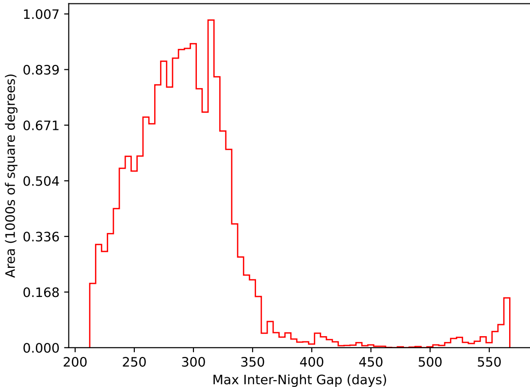
ddf_acor_sf10_lsf20_lsr50_v3.4_10yrs WFD i band: Max Inter-Night Gap
