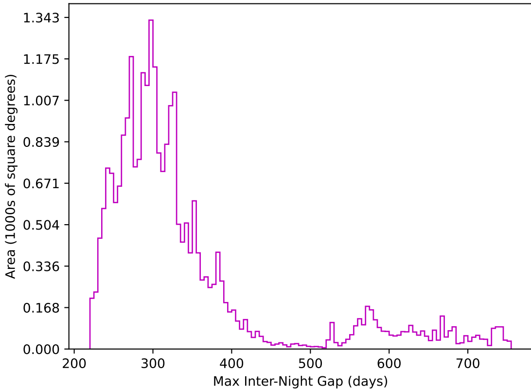
ddf_acor_sf10_lsf20_lsr50_v3.4_10yrs All sky z band: Max Inter-Night Gap
