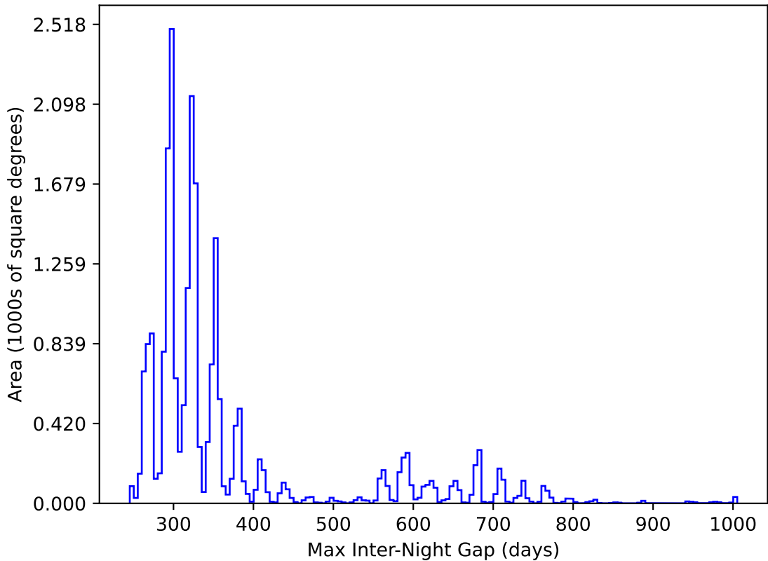
ddf_acor_sf10_lsf20_lsr50_v3.4_10yrs All sky y band: Max Inter-Night Gap
