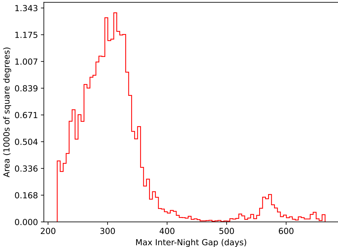
ddf_acor_sf10_lsf20_lsr50_v3.4_10yrs All sky i band: Max Inter-Night Gap
