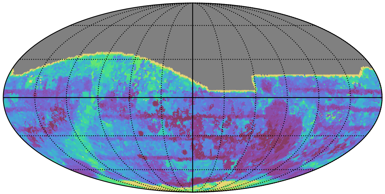
ddf_acor_sf10_lsf20_lsr50_v3.4_10yrs All sky all bands: Max Inter-Night Gap
