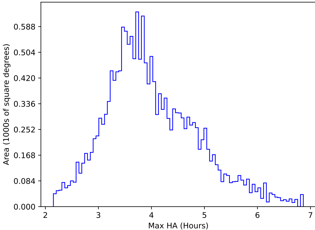
ddf_acor_sf10_lsf20_lsr50_v3.4_10yrs WFD u band: Max HA
