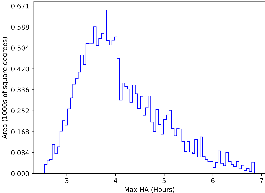
ddf_acor_sf10_lsf20_lsr50_v3.4_10yrs WFD g band: Max HA
