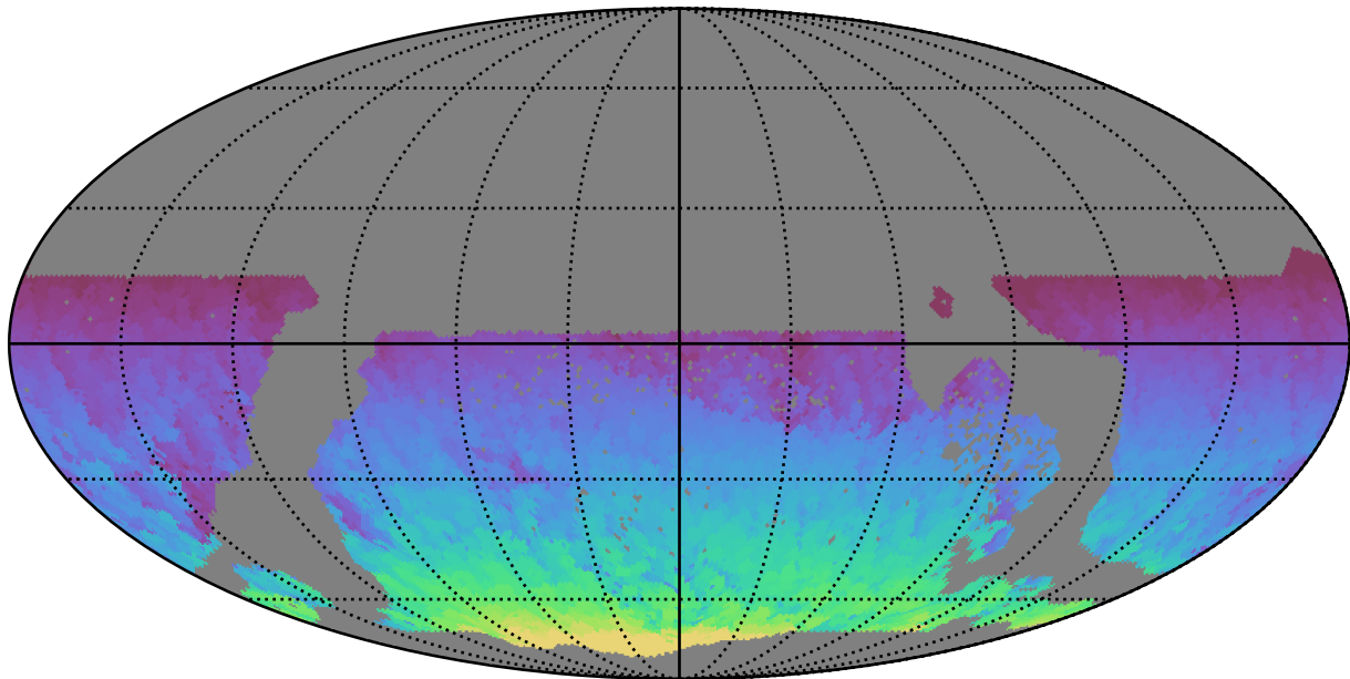
ddf_acor_sf10_lsf20_lsr50_v3.4_10yrs WFD all bands: Max HA
