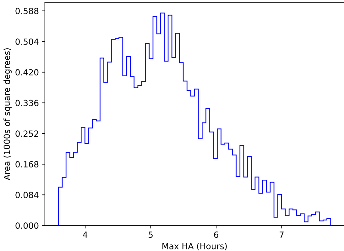
ddf_acor_sf10_lsf20_lsr50_v3.4_10yrs WFD all bands: Max HA
