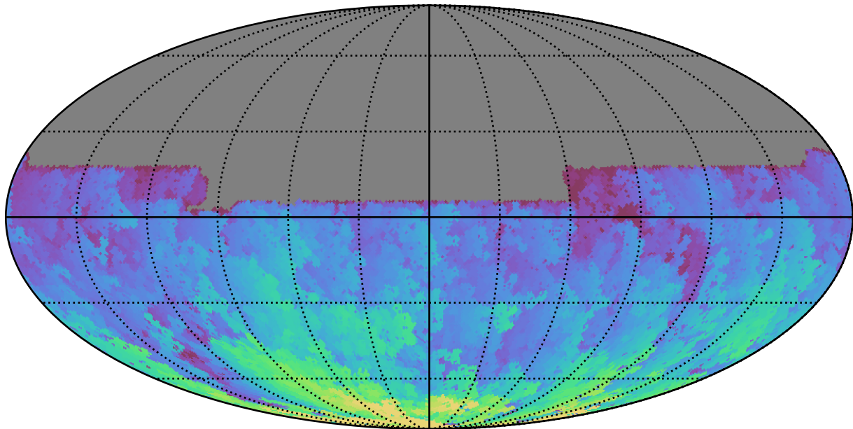
ddf_acor_sf10_lsf20_lsr50_v3.4_10yrs All sky u band: Max HA
