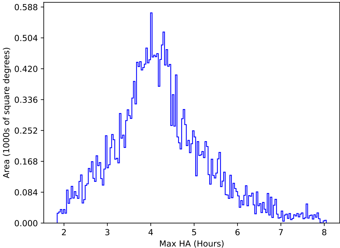
ddf_acor_sf10_ls20_lsr50_v3.4_10yrs All sky r band: Max HA
