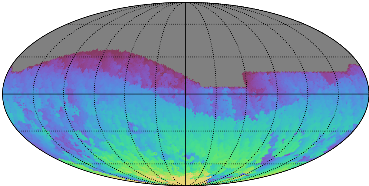
ddf_acor_sf10_lsf20_lsr50_v3.4_10yrs All sky i band: Max HA
