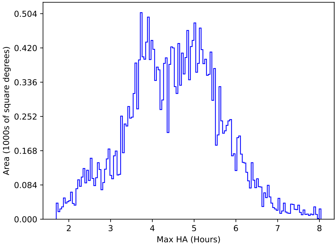
ddf_acor_sf10_ls20_lsr50_v3.4_10yrs All sky i band: Max HA
