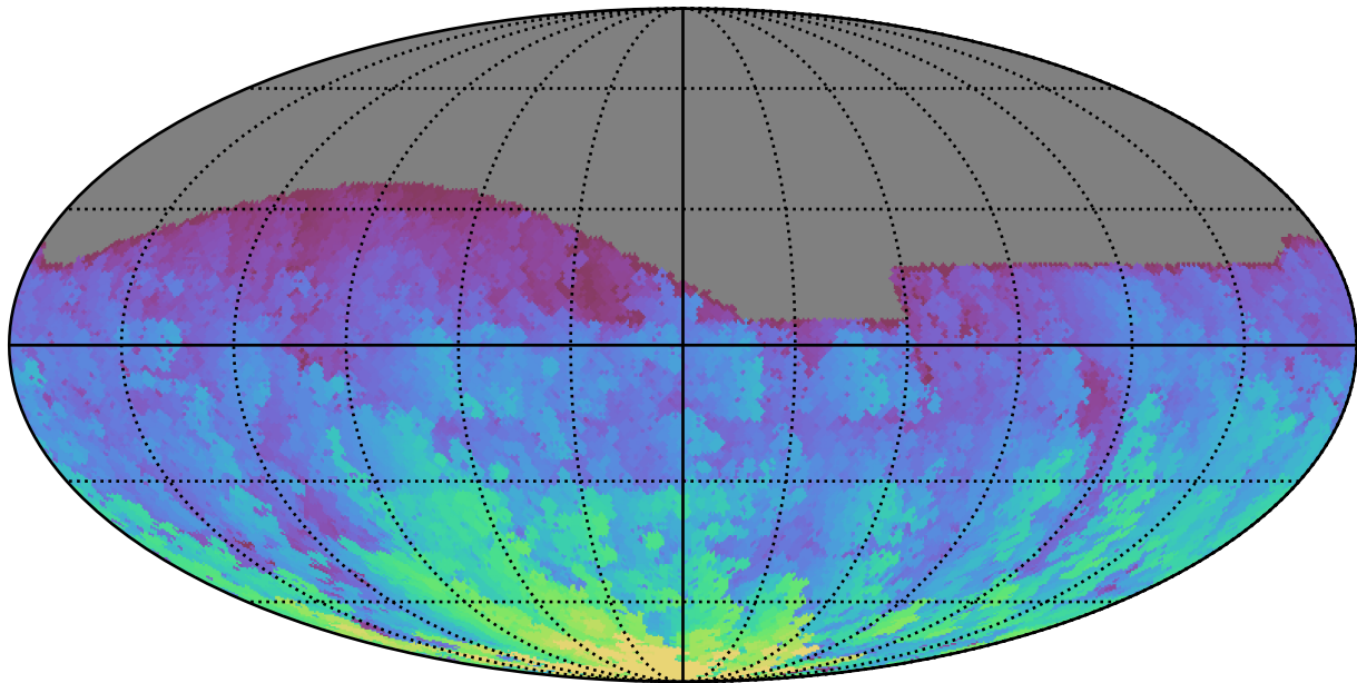
ddf_acor_sf10_lsf20_lsr50_v3.4_10yrs All sky g band: Max HA
