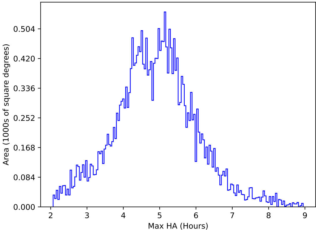
ddf_acor_sf10_lsf20_lsr50_v3.4_10yrs All sky all bands: Max HA
