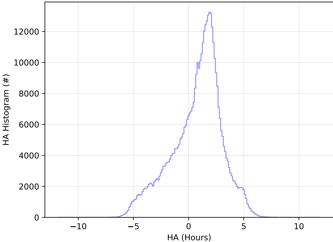
ddf_acor_sf10_lsf20_lsr50_v3.4_10yrs WFD z band: HA Histogram
