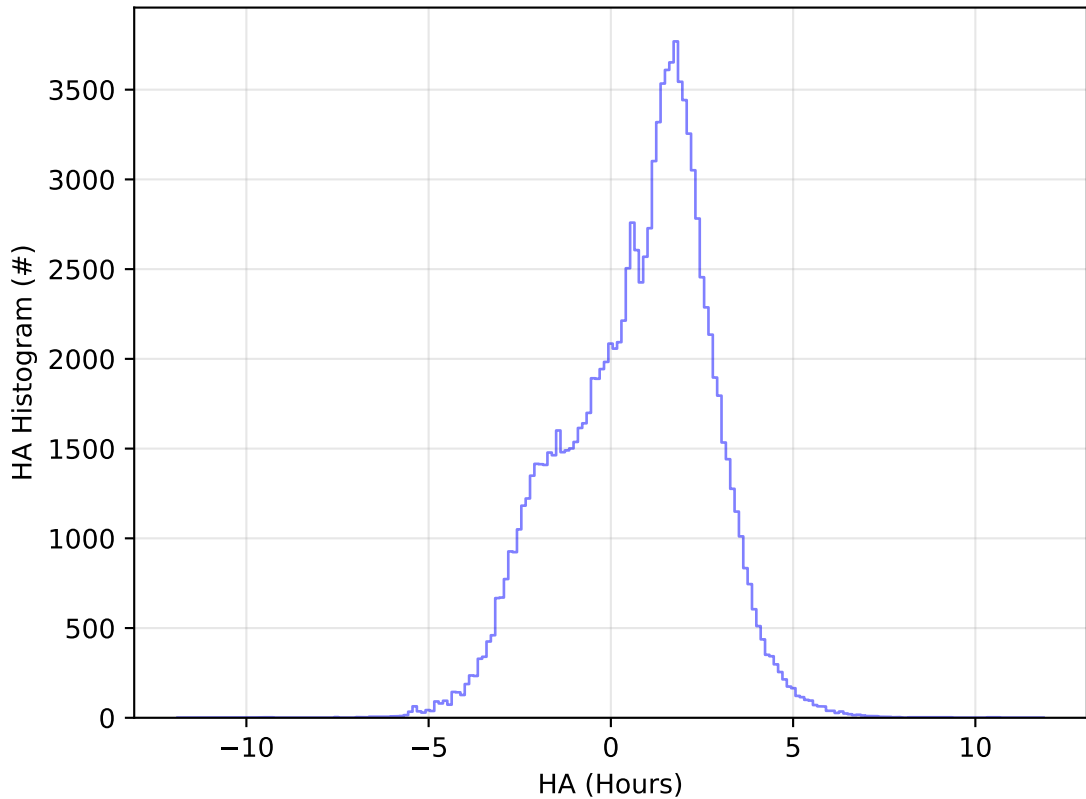
ddf_acor_sf10_lsf20_lsr50_v3.4_10yrs WFD u band: HA Histogram
