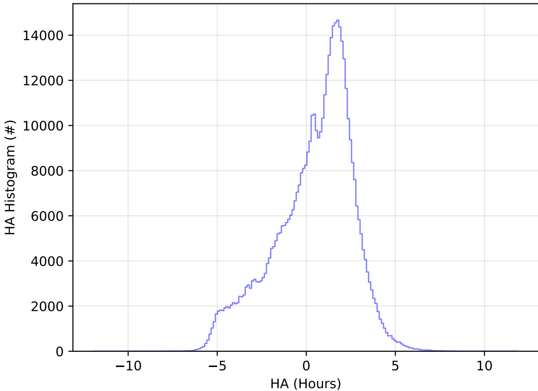
ddf_acor_sf10_lsf20_lsr50_v3.4_10yrs WFD r band: HA Histogram
