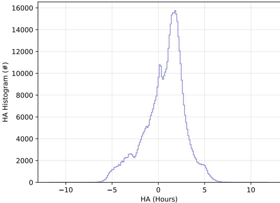
ddf_acor_sf10_lsf20_lsr50_v3.4_10yrs WFD i band: HA Histogram
