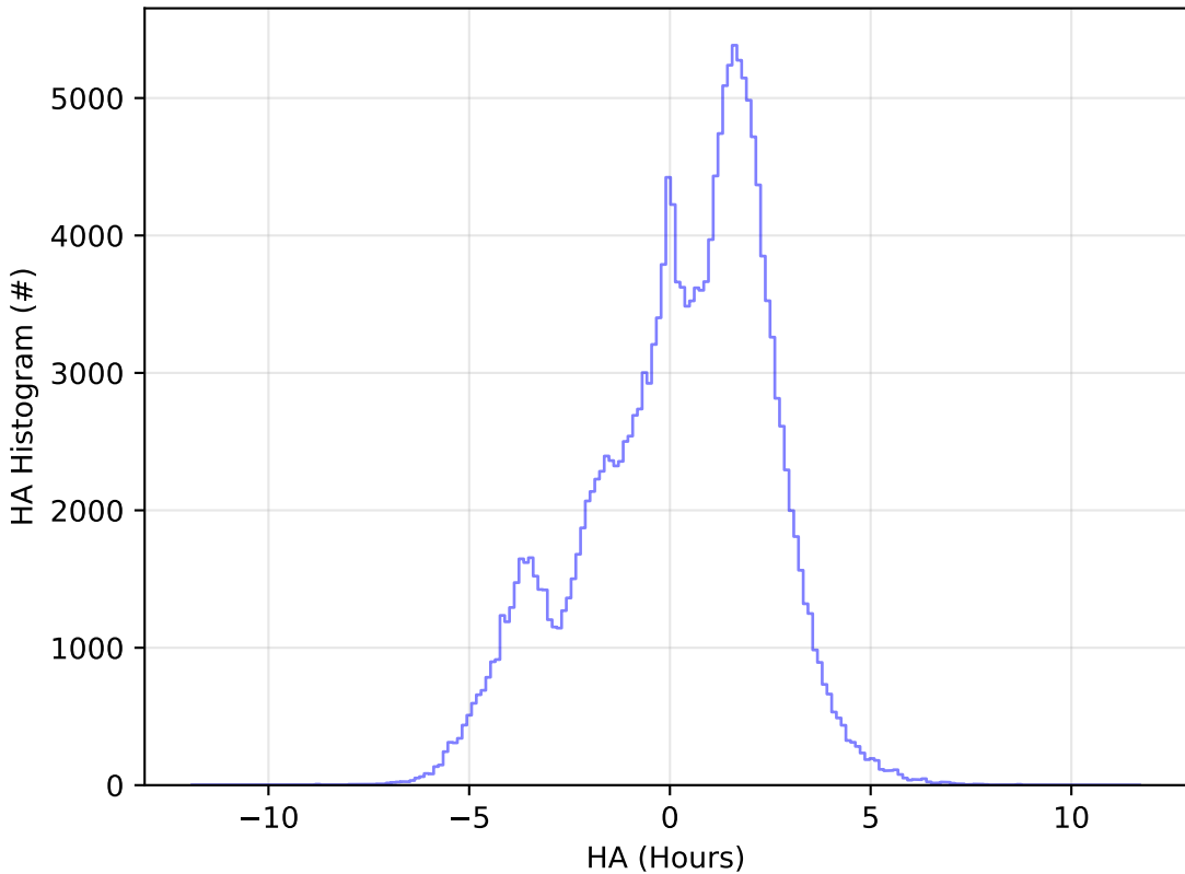
ddf_acor_sf10_lsf20_lsr50_v3.4_10yrs WFD g band: HA Histogram
