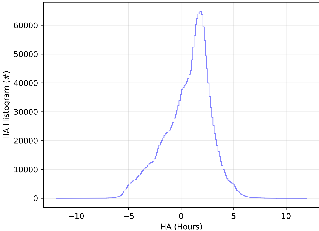
ddf_acor_sf10_lsf20_lsr50_v3.4_10yrs WFD all bands: HA Histogram
